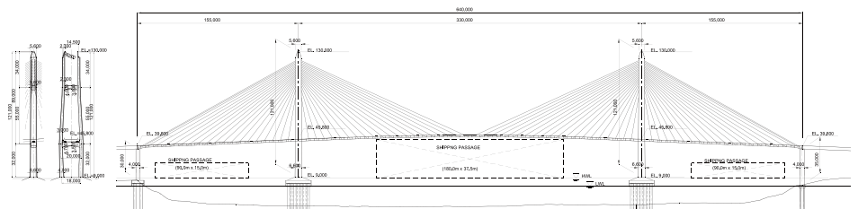
General Drawing
